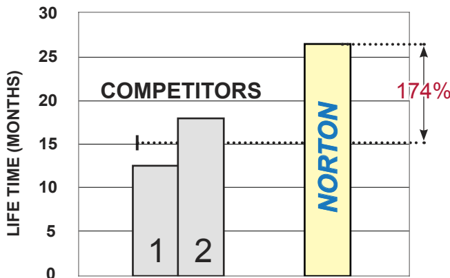
Average Life Time of the Pulpstone removed from PGW Grinders
